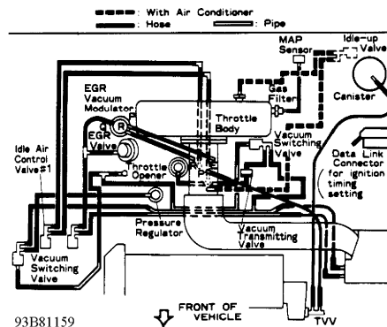
Fig. 29: Vacuum Diagram (Tercel - Calif. Models W/O Power Steering) Courtesy of Toyota Motor Sales, U.S.A., Inc.
