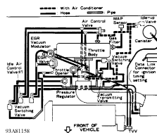
Fig. 28: Vacuum Diagram (Tercel - Calif. Models W/ Power Steering) Courtesy of Toyota Motor Sales, U.S.A., Inc.
